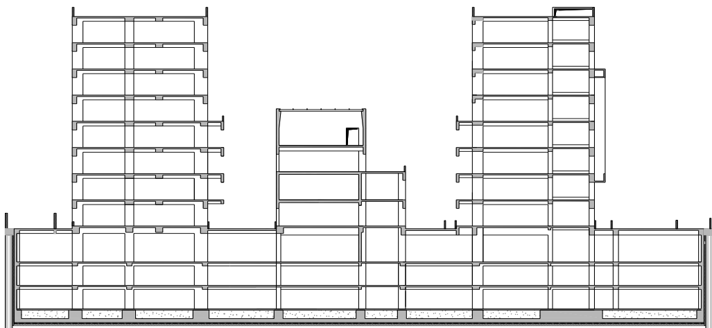
Structural framing cross section
