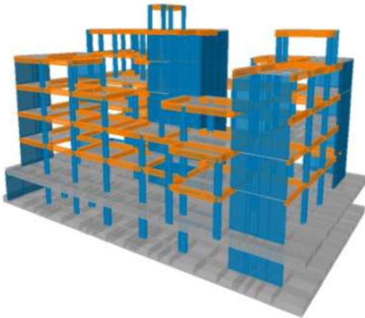
ETABS structural model of typical apartment building
