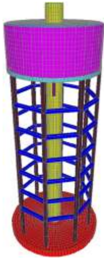
Structural Model of 500 cu.m. Elevated Water Tank
